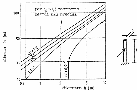
Fig. C.7.11 (c) - ciminiere in c.a.
